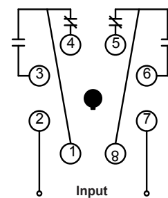
Octal Base
