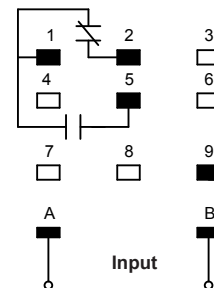
Square Base
