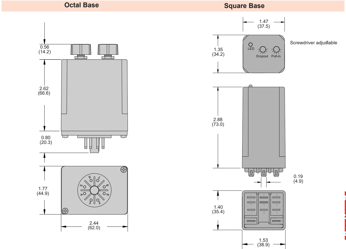
Max Outline Dimensions Dimensions Shown in inches & (millimeters)
