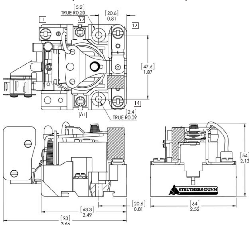
450XAX (SPDT - 1 FORM C)
